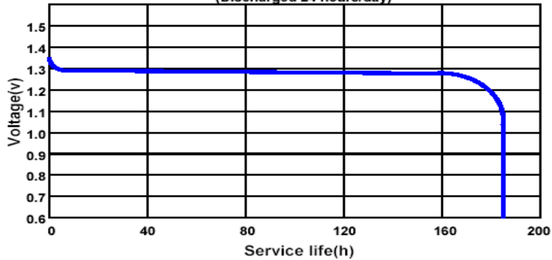
MINIMUM DISCHARGE CHARACTERISTICS AT 3KΩ 25°C 60%RH (Discharged 24 hours/day)
